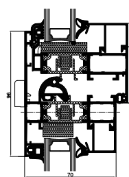
Opening window and fixed window – cross-section
